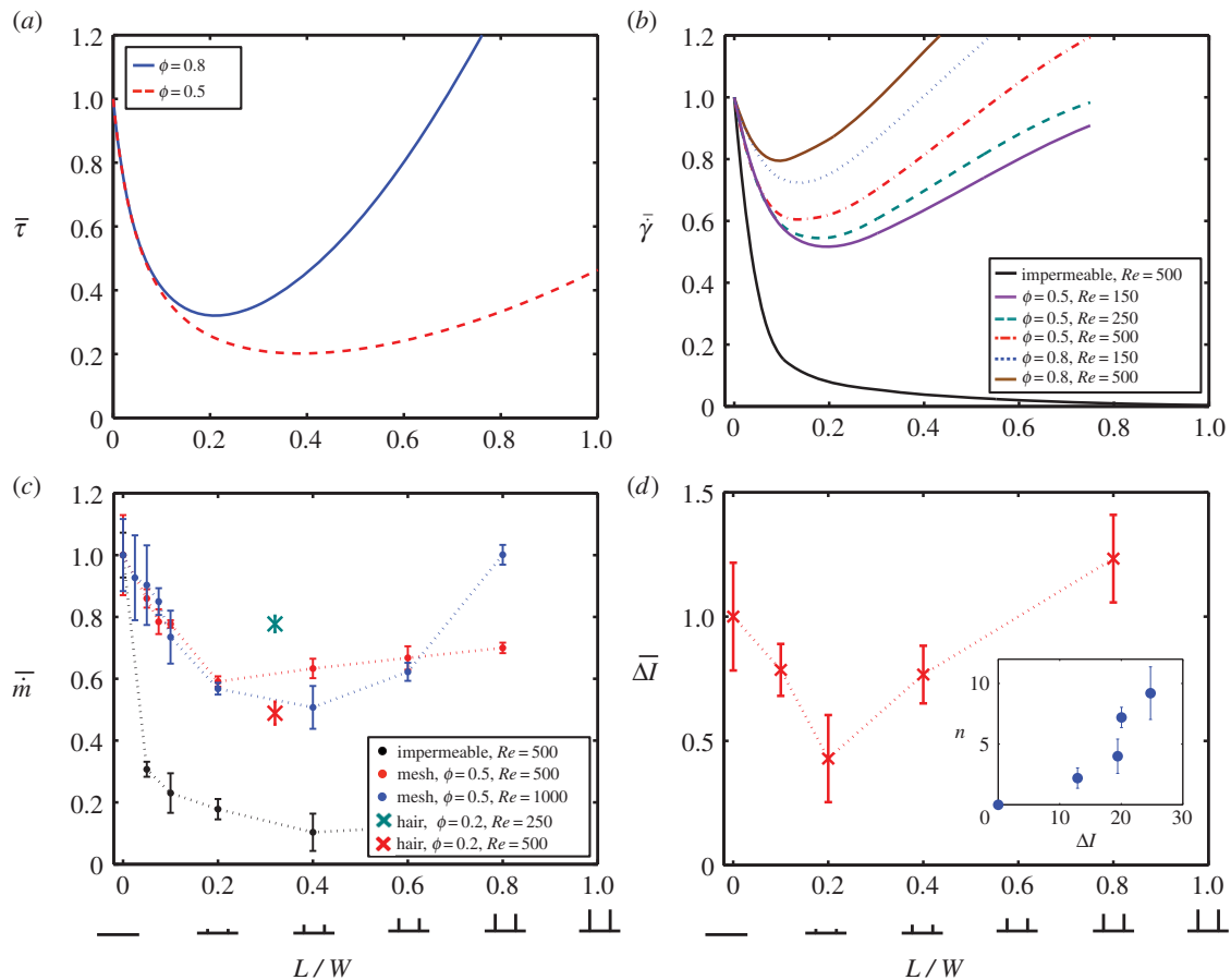
Figure 8. (a) Shear stress \bar{\tau} , (b) shear rate \bar{\gamma} , (c) evaporation rate \bar{m} , and (d) change in fluorescence intensity \bar{\Delta I} , all versus eyelash length L/W . All values reported are normalized with their respective values for an eye with no lashes. (d) Inset shows relationship between number of deposited drops n in drops \text{mm}^{-2} and change in fluorescence intensity \Delta I . (Online version in colour.)
