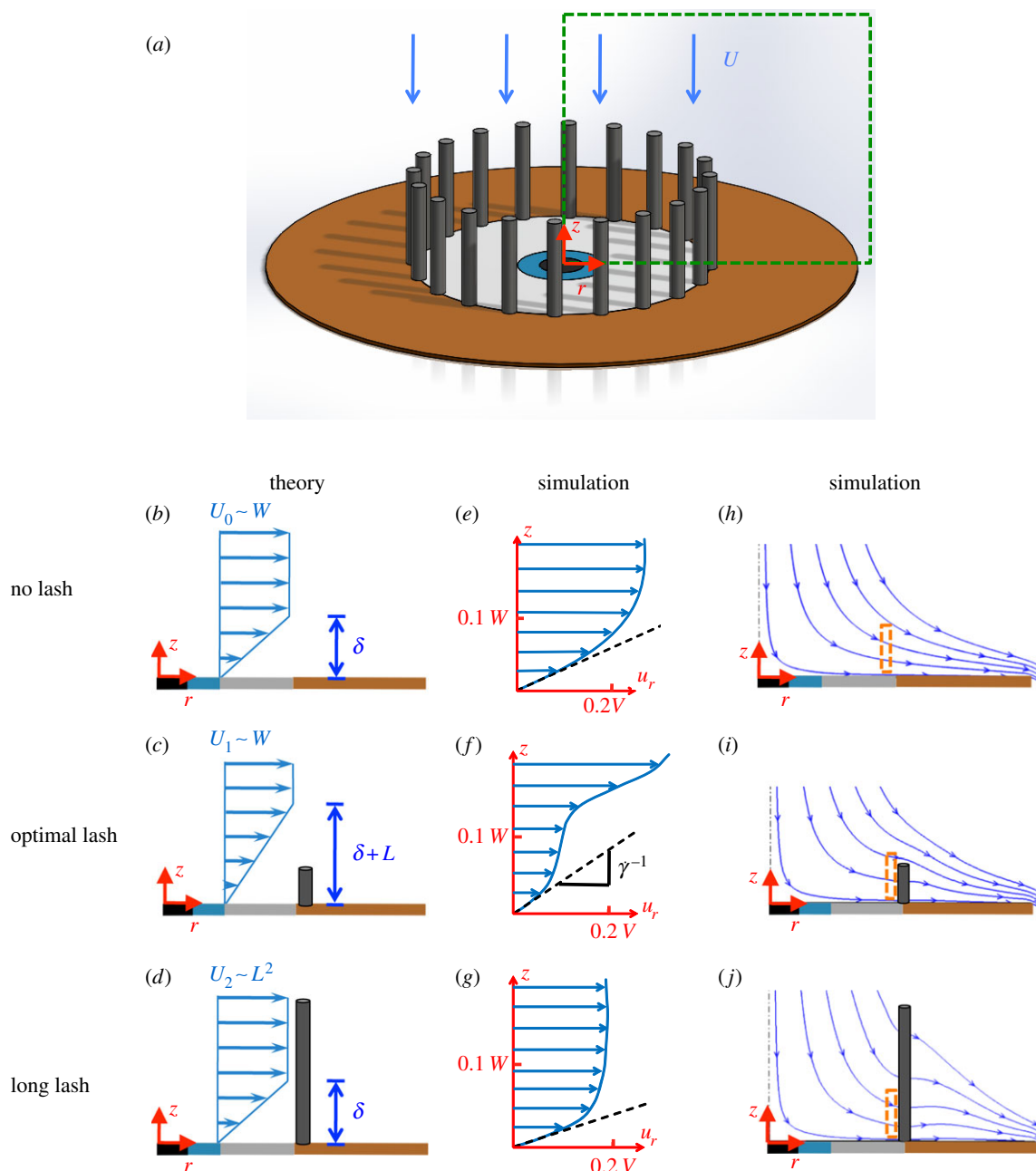
Figure 7. Velocity near the eye. (a) Dashed box shows cross section of flow from which velocity is shown. Columns show both theoretical (b–d) and (e–g) numerical predictions for the radial velocity u_r distribution along the height z above the ocular surface. (h–j) The final column shows numerical predictions for streamlines. The dashed box shows the location of the velocity profiles in (e–g). Rows represent the three cases: no lashes, optimal lashes and long lashes. (Online version in colour.)
